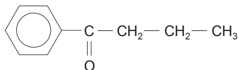
1-phenylbutanone
